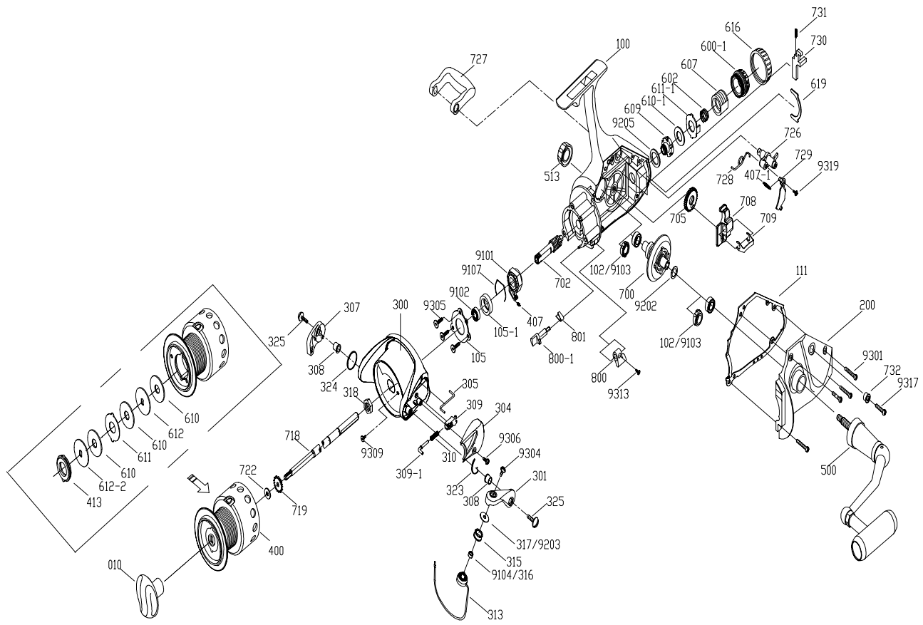
CD - 50 Spare Parts
